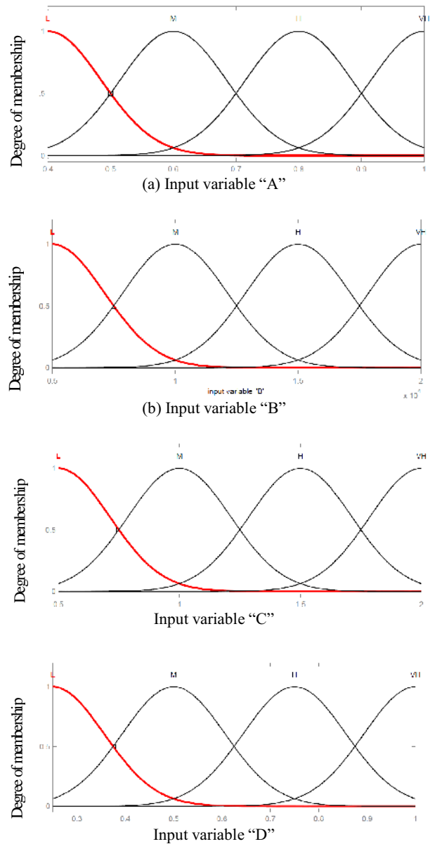
Fig. 5 Membership function for variables of inputs
