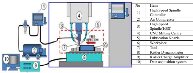
Fig. 2 The experimental set-up
