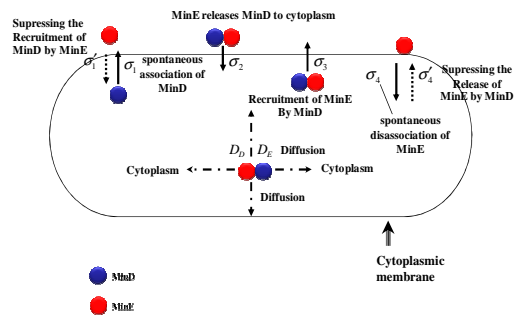
Fig. 1 A schematic diagram of the MinD/MinE dynamics which was proposed by Howard et al. (2001)
