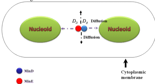
Fig. 2 A schematic diagram of the MinD/MinE dynamics with nucleoid zones
