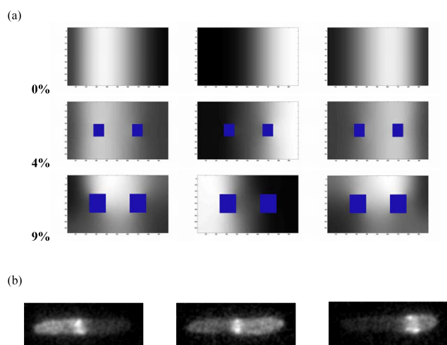
Fig. 6 MinE dynamics from the LBM and experiment. (a) The numerical results of MinE dynamics for different conditions of obstacles. The obstacles are shown at 0,4,9 percents of cell size. (b) The experimental results of MinE proteins are shown in terms of fluorescent intensity [26, 27]. The MinE clusters are observed near the cytoplasmic membrane
