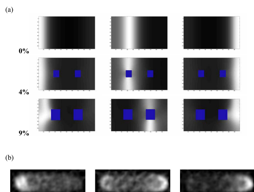
Fig. 5 MinD dynamics from LBM and experiment. (a) The numerical results of MinD dynamics for different conditions of obstacles. The obstacles are shown at 0,4,9 percents of cell size. (b) The experimental results of MinD protein are shown in term of fluorescent intensity [26, 27]. The MinD clusters are observed near the cytoplasmic membrane
