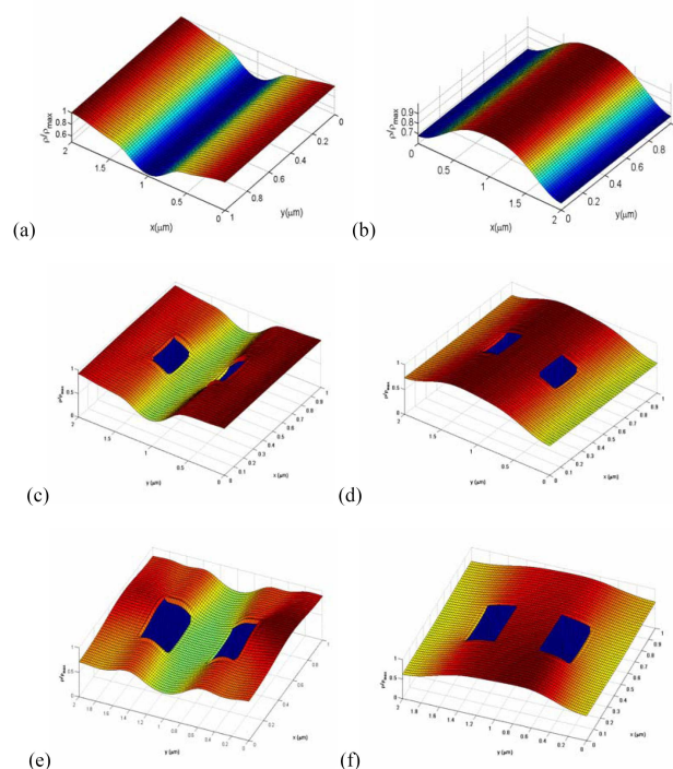
Fig. 7 Time-average plots of MinD and MinE dynamics from the LBM with and without obstacles. The MinD protein is shown in terms of the time-averaged density for the obstacles 0,4,9 percents of cell size as shown in (a), (c), (e), respectively. The MinE protein is shown in terms of time-averaged density for the obstacles 0,4,9 percents of cell size as shown in (b), (d), (f), respectively
