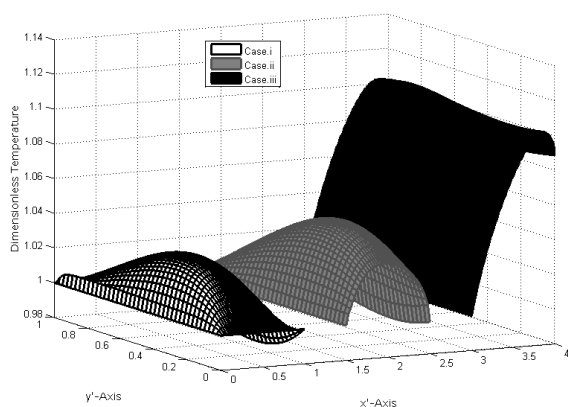
Fig. 3 Dimensionless temperature distributions for transverse roughness ( m=0.4, T_1=1.0 )
