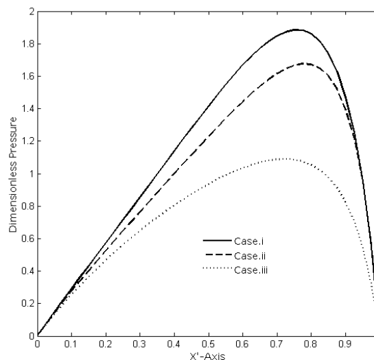
Fig. 4 Dimensionless pressure distributions for transverse roughness ( m=0.4, T_1=1.0 )
