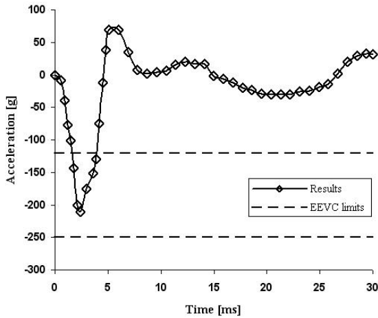
Fig. 18 Upper tibia acceleration in dynamic certification test
