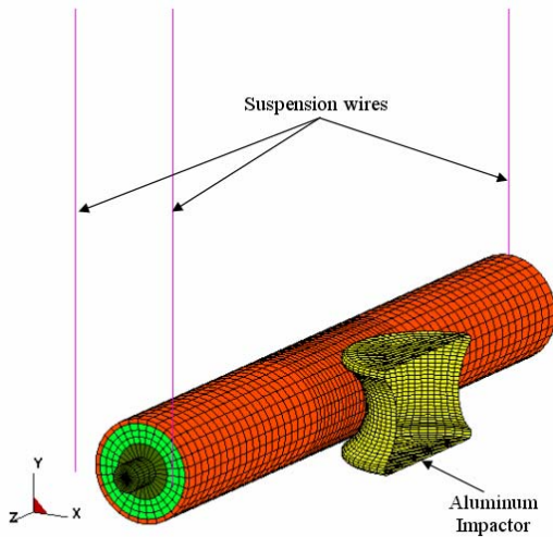
Fig. 14 Dynamic certification test
