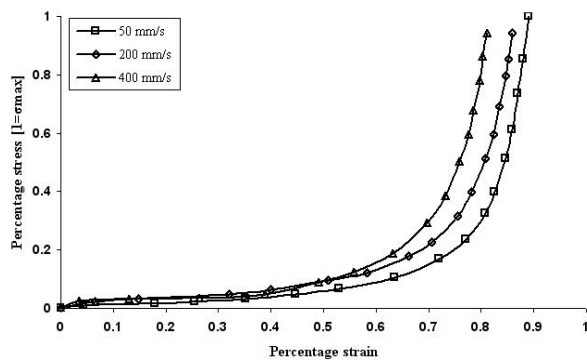
Fig. 4 Foam test results [10]
