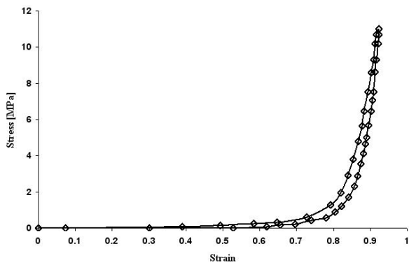
Fig. 5 Neoprene stress strain curve [11]
