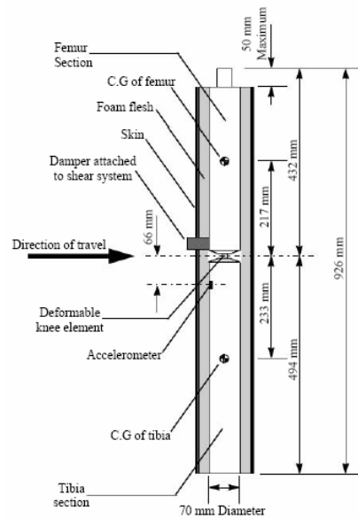
Fig. 3 Legform impactor with skin and foam covering [2]
