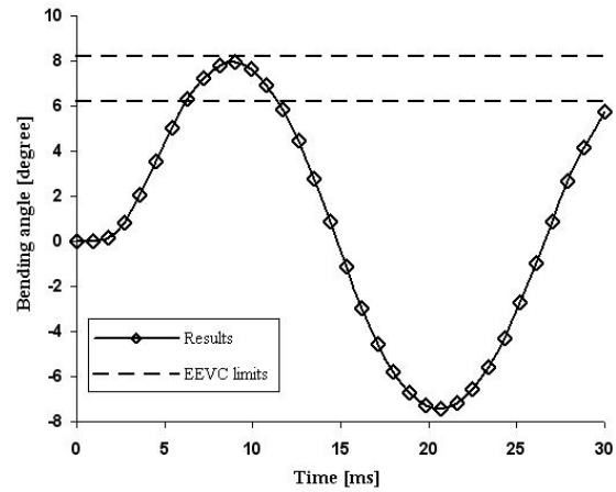
Fig. 16 Knee bending angle in dynamic certification test
