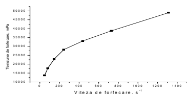
Fig. 2 Rheogram of gel with collagen concentration of 0,6%, without ethyl alcohol
