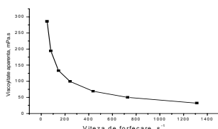
Fig. 7. Fluctuation of apparent viscosities with shearing speeds for the gel containing 10% of 70% ethyl alcohol solution.
