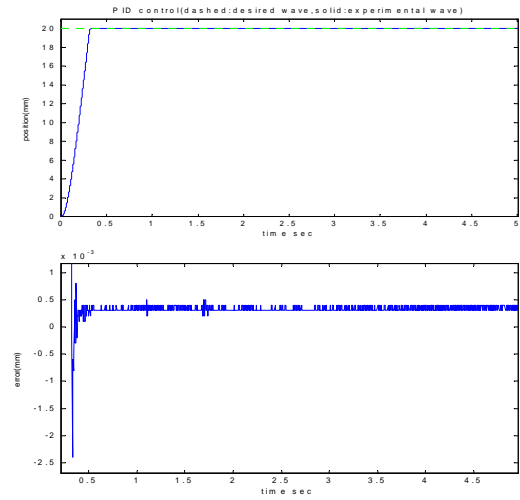
Fig. 5 PID control step response and error history
