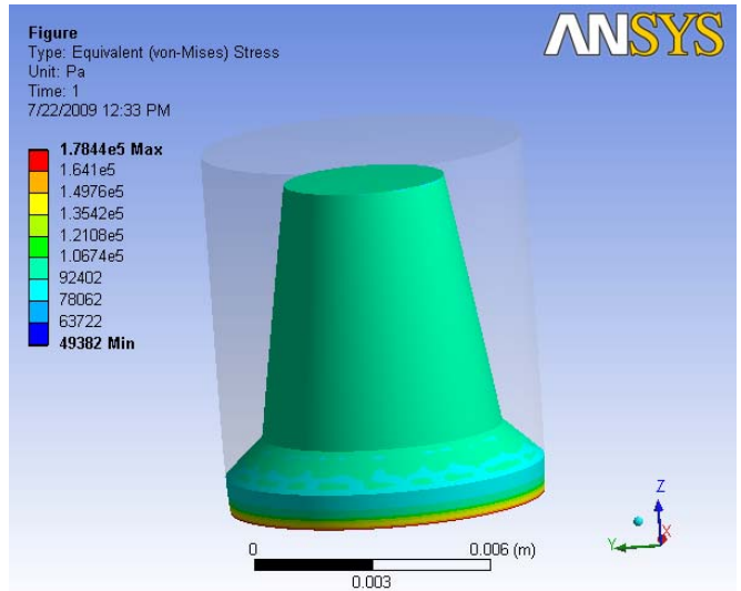
Fig. 7 Maximal equivalent stress in a tooth preparation with sloped shoulder margin (fine simulation)
