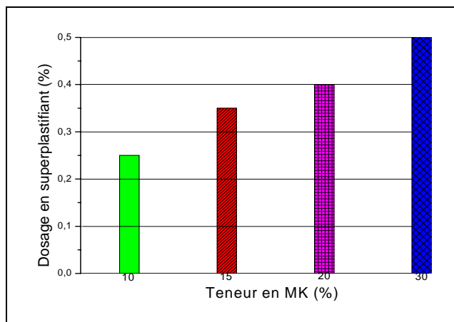
Fig. 1 Effect of MK content on superplasticizer demand
