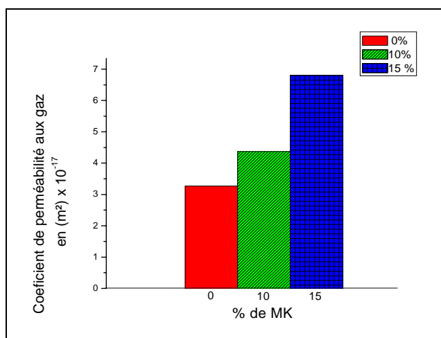
Fig. 9 Effect of metakaolin on gas permeability
