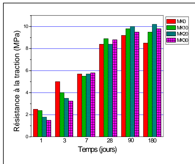
Fig. 3 Development of the flexural strength of mortar with time
