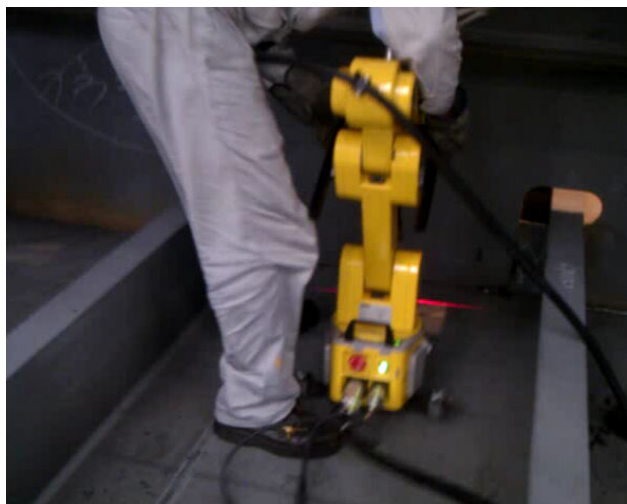
Fig. 9 Handling and setting of the developed robot
