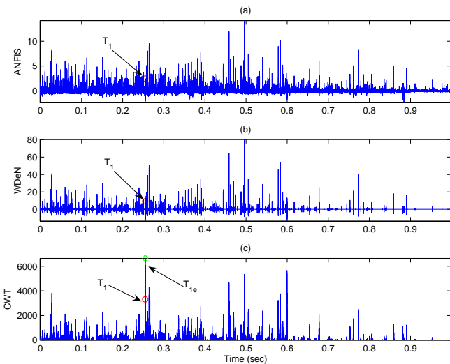
Fig. 4. (a)ANC neuro-fuzzy output of the 1^{st} target ping T_1 with 5 ANFIS epochs. (b)Output of the 1^{st} WDeN without TM-levelization. (c) Output of the 1^{st} optimal CWT mapping: |f^3(s_1^*) - f^0(s_1^*)| .
