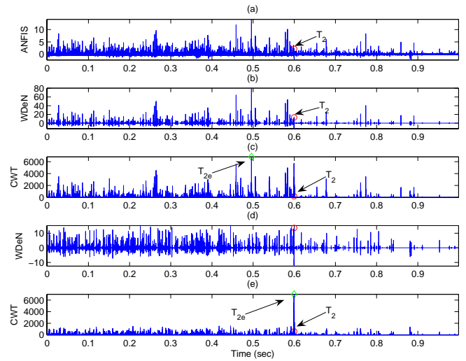
Fig. 5. (a)ANC neuro-fuzzy output of the 2^{nd} target ping T_2 with 5 ANFIS epochs. (b)Output of the 1^{st} WDeN without TM-levelization. (c) Output of the 1^{st} optimal CWT mapping: |f^3(s_1^*) - f^0(s_1^*)| . (d) Output of the 2^{nd} WDeN with TM_{\alpha_1} = TM_{\alpha_2} = 7.5 \times 10^{-4} . (e) Output of the 2^{nd} optimal CWT mapping: |f^3(s_2^*) - f^0(s_2^*)| .
