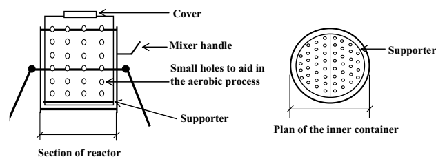
Fig. 1 The aerobic compost reactor
