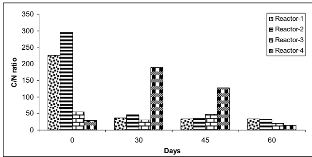
Fig. 9 Variations of C/N ratio during composting
