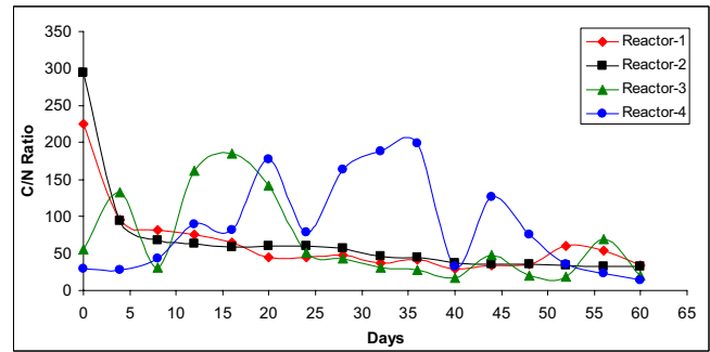
Fig. 8 Variations of C/N ratio during composting
