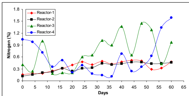
Fig. 7 Variations of nitrogen during composting
