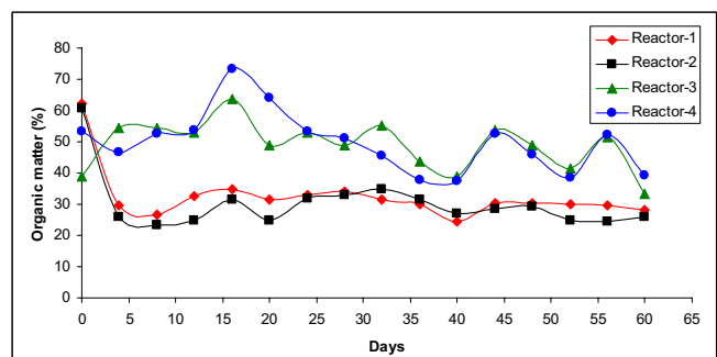
Fig. 5 Variations of organic matter during composting
