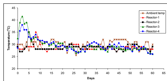
Fig. 2 Variations of temperature during composting
