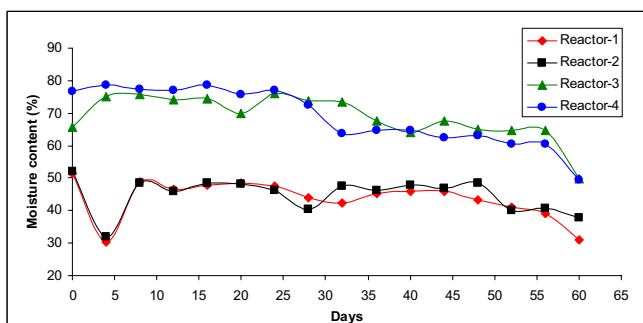
Fig. 4 Variations of moisture content during composting
