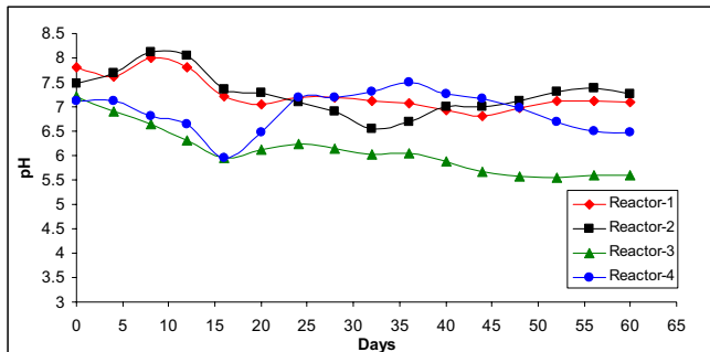
Fig. 3 Variations of pH during composting
