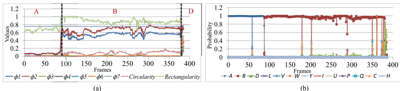
Fig. 5: (a) Graph shows the statistical and geometrical feature vector set of the posture signs 'A', 'B' and 'D'. (b) Classification probability of the test sequence. Blue curve shows the highest probability in the initial frames which classifies 'A'; classification for 'B' sign is shown by the brown curve and 'D' is shown in the last frames by light green curve.
