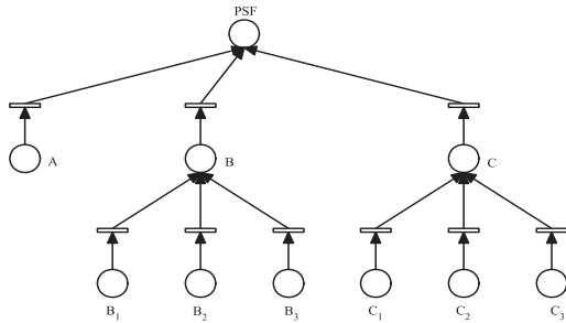
Fig. 3. Petri net model of press unit
