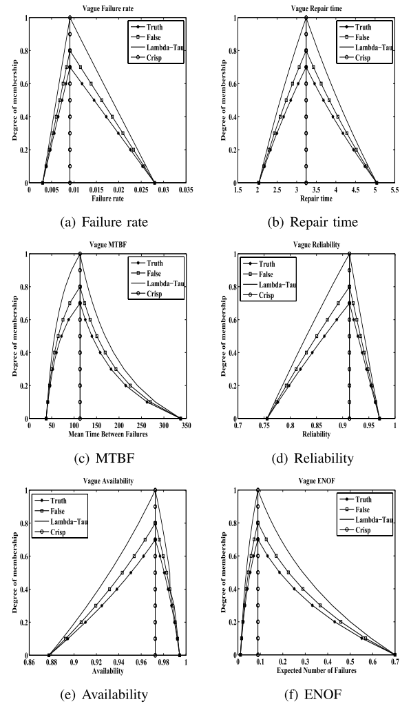
Fig. 5. Vague reliability parameters plots for press system
