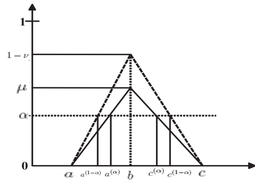
Fig. 2. \alpha - cut of IFS \tilde{A}
