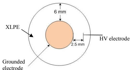
Fig. 2 Schematic diagram of specimen
