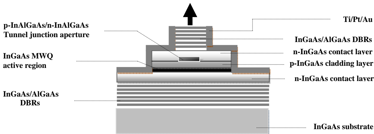
Fig. 1 Basic device structure of the proposed top emitting VCSEL.
