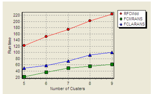
Fig. 9 Runtime for different cluster count on sample from NG of size 2500
