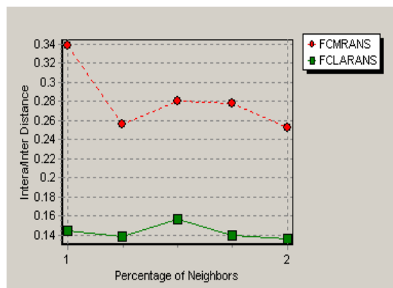
Fig. 2 Intra/Inter distance for different values for maxneighbor
