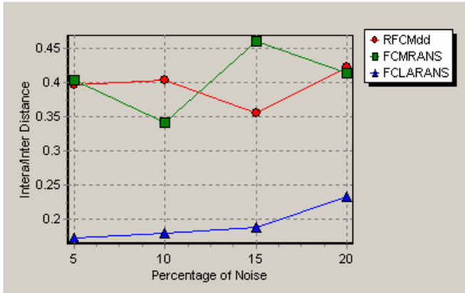
Fig. 6 Intra/Inter Cluster distance for different noise levels
