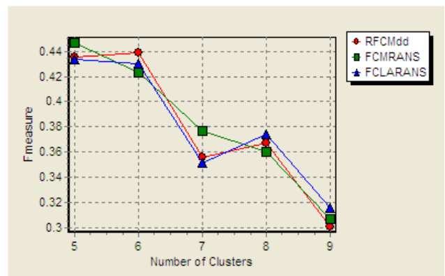
Fig. 10 F-measure for different cluster count on from NG of size 2500
