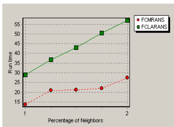
Fig. 1 Runtime for Different values for maxneighbor
