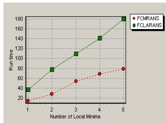
Fig. 3 Runtime for different values for numlocal
