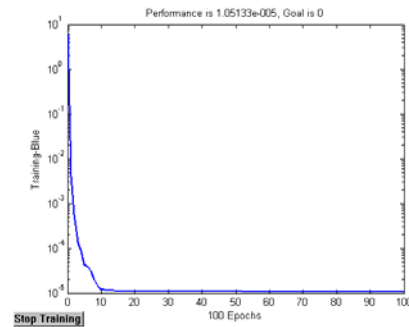
Fig. 6 Training phase
