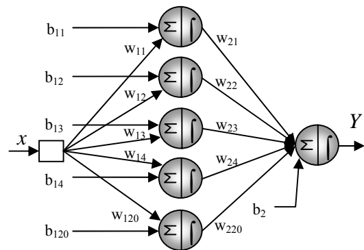
Fig. 5 Network architecture
