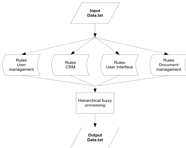
Fig. 4 Hierarchical structure processing
