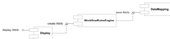
Fig. 6 Atom workflow
