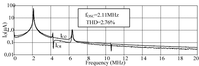
Fig. 5 Frequency spectrum of signal in Fig. 4
