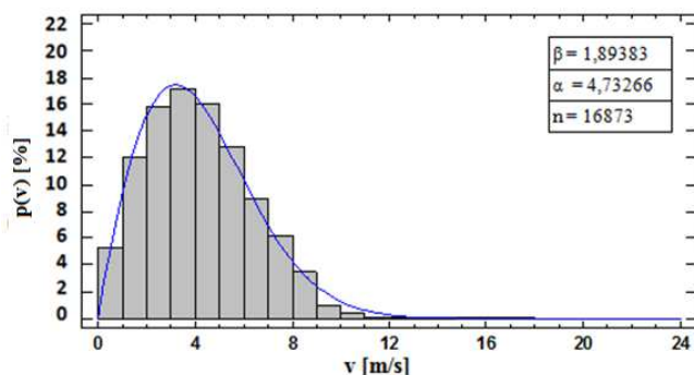
Fig. 23 Weibull distribution of the average wind speed during May 2011
