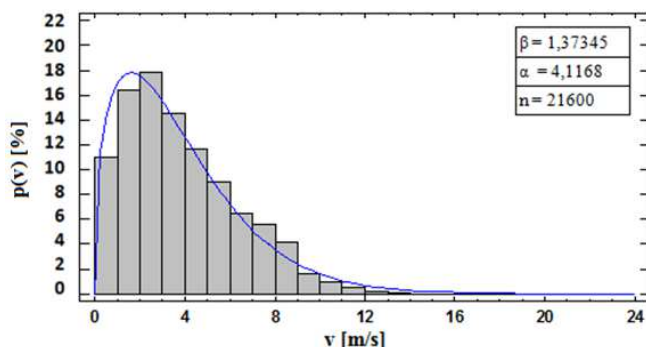
Fig. 29 Weibull distribution of the average wind speed during November 2011
