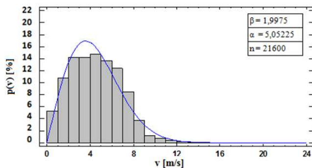
Fig. 22 Weibull distribution of the average wind speed during April 2011
