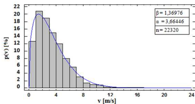
Fig. 30 Weibull distribution of the average wind speed during December 2011
