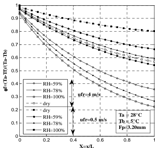
Fig. 2 Effect of relative humidity on the fin temperature distribution
