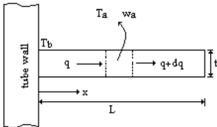
Fig. 1 Schematic diagram of a rectangular fin
