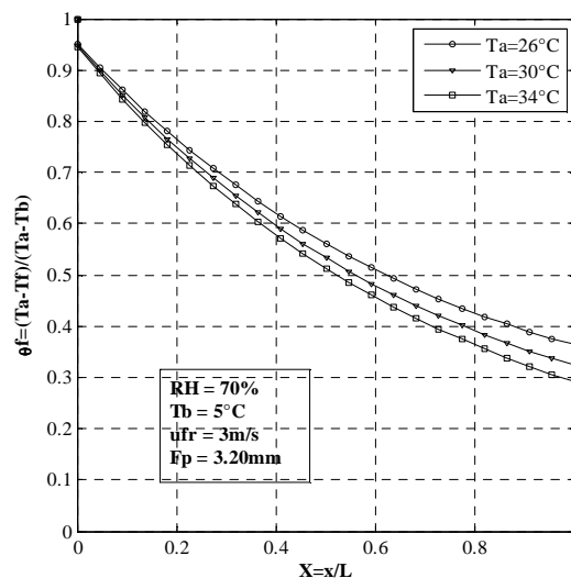
Fig. 3 Effect of dry bulb temperature on the temperature distribution
