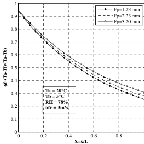
Fig. 5 Effect of fin pitch on the temperature distribution
