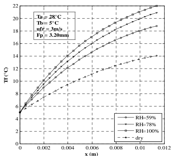
Fig. 4 distribution of fin temperature
