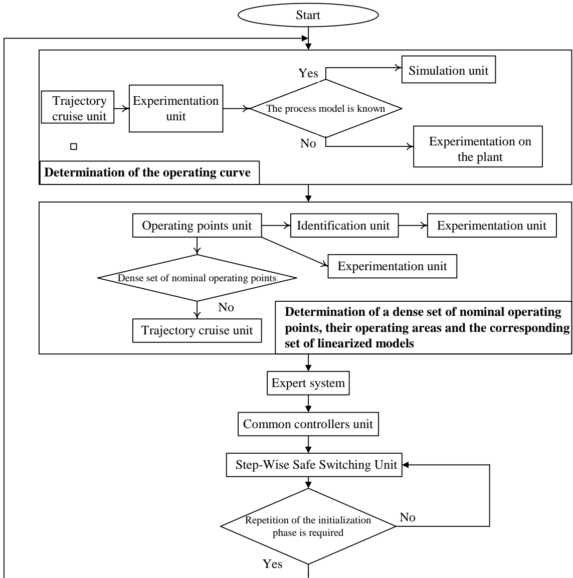
Fig. 1 Flow chart of the Supervisory Scheme
