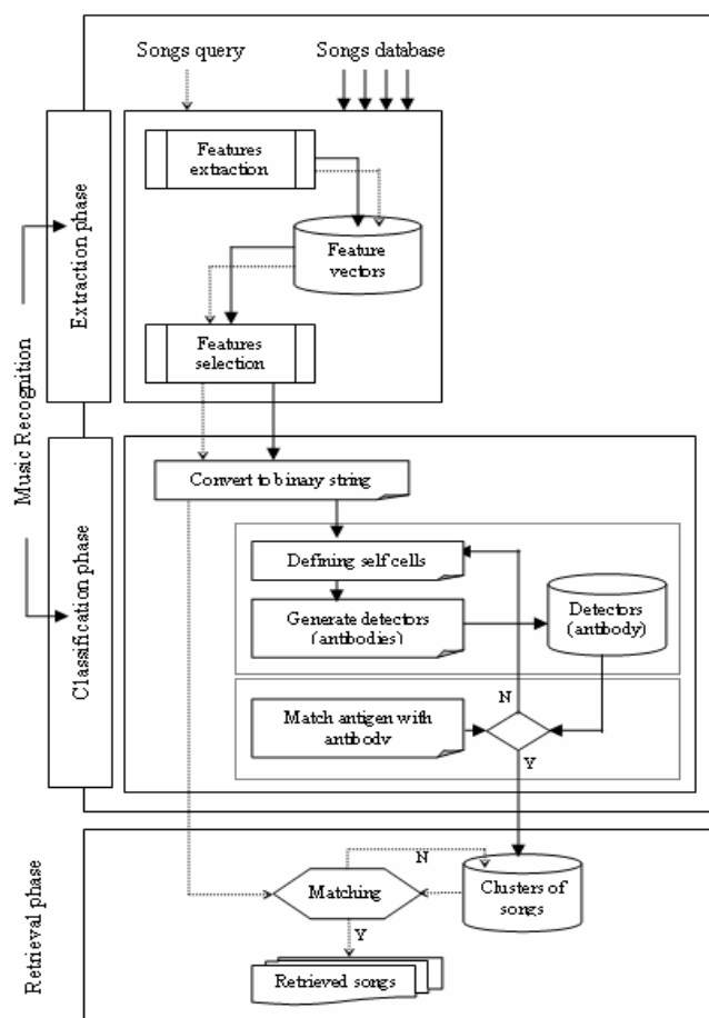
Fig. 1 Proposed Audio Content-Based Retrieval Framework
