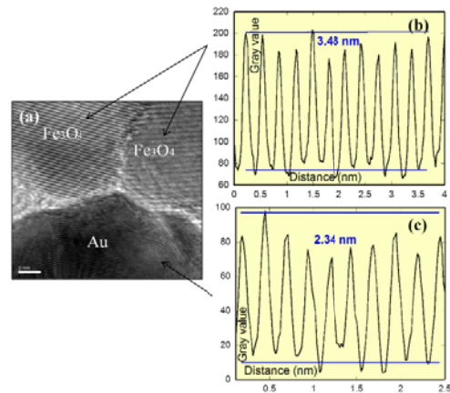
Fig. 4 HR-TEM results (a) high magnification view of \text{Au}@Fe_3O_4 nanoparticles (b) line profile image contrast for \text{Fe}_3\text{O}_4 and (c) for Au
