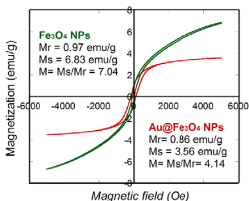
Fig. 6 Hysteresis loop of magnetization ( M , emu g^{-1} ) versus magnetic field ( H , Oe) for magnetite (Fe 3 O 4 ) and Au@Fe 3 O 4 nanoparticles
