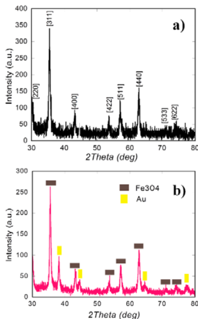
Fig. 2 XRD patterns of \text{Fe}_3\text{O}_4 (a) and \text{Au}@Fe_3O_4 (b) nanoparticles synthesized by pulsed plasma in liquid
