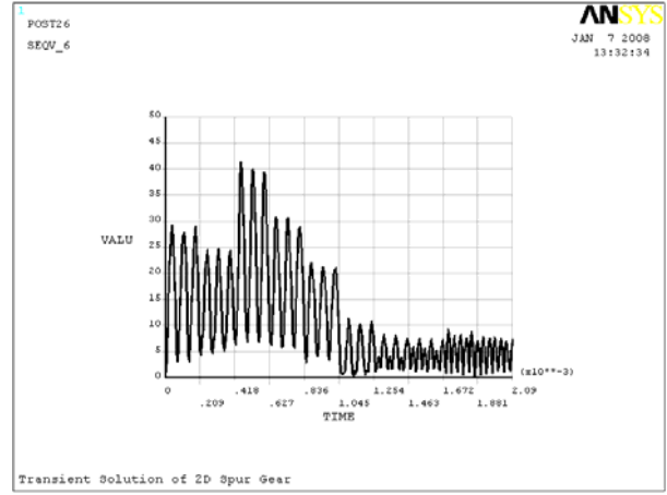
Fig. 12 Dynamic von Mises Stress of the model
