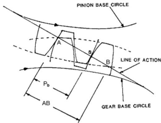
Fig. 4 Contact path
