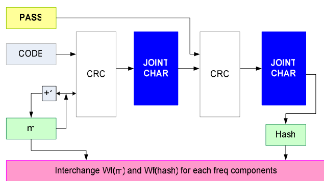
Fig 5 Transverse using CRC-32 Hash function
