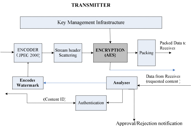
Fig 2 Transmitter LSI with encryption method
