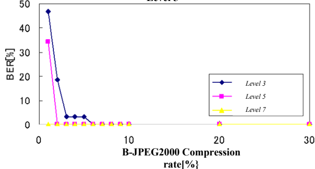
Fig 10 Embedded Data under Compression
