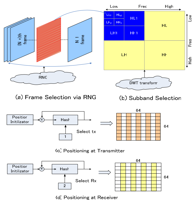
Fig 6 Watermarking Algorithm
