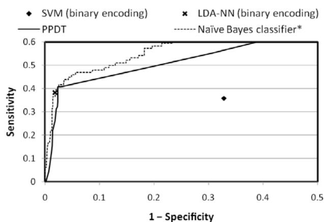
Fig. 2 Performance comparisons of PPDT and SVM and LDA-NN methods based on binary encoding
