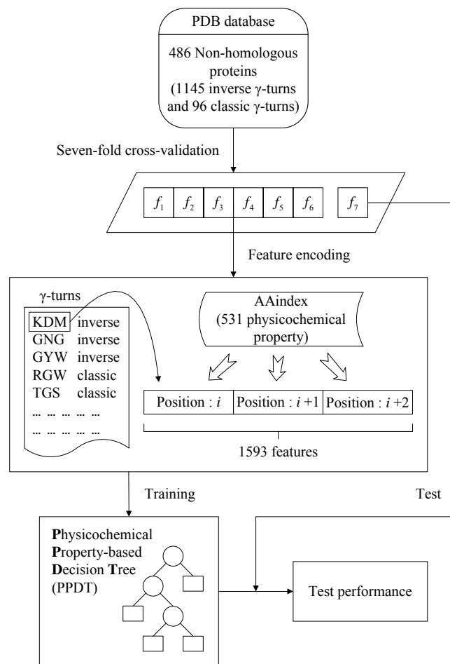
Fig. 1 System flow of the proposed PPDT method.
