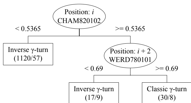
Fig. 3 Physicochemical property-based decision tree.
