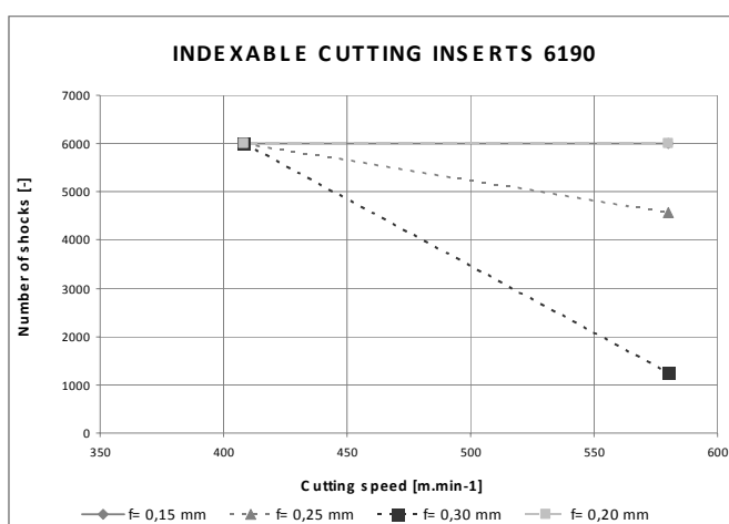
Fig. 7 Dependence – the number of shocks on cutting speed
