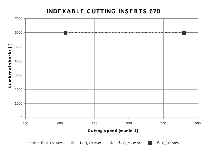
Fig. 9 Dependence – the number of shocks on cutting speed
