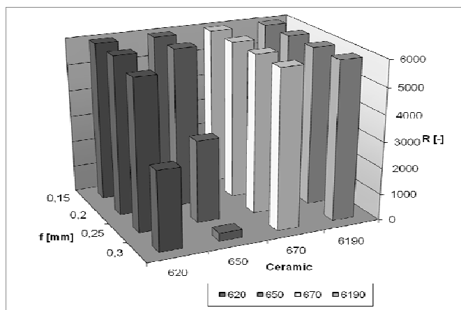
Fig. 14 Dependence – the number of shocks on feed – cutting speed v_c = 408 \text{ m.min}^{-1}
