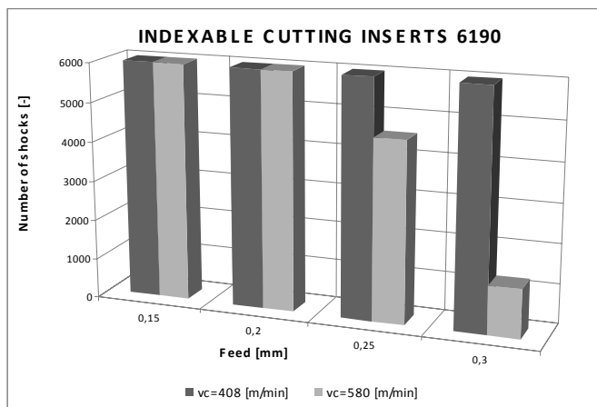
Fig. 6 Dependence – the number of shocks on feed
