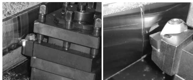
Fig. 5 Toolholder CSRNR 25x25M12- K
