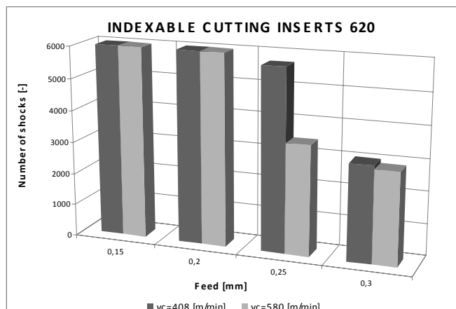
Fig. 12 Dependence – the number of shocks on feed
