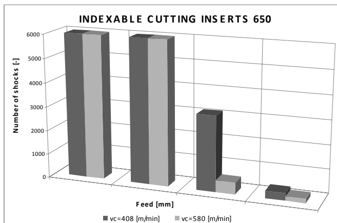
Fig. 10 Dependence – the number of shocks on feed
