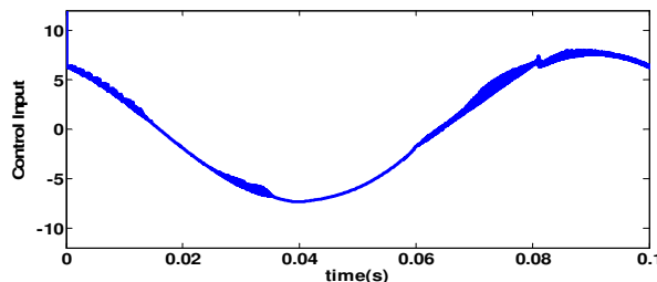
Fig. 11. Control Signal without Fuzzy gain Tuning
