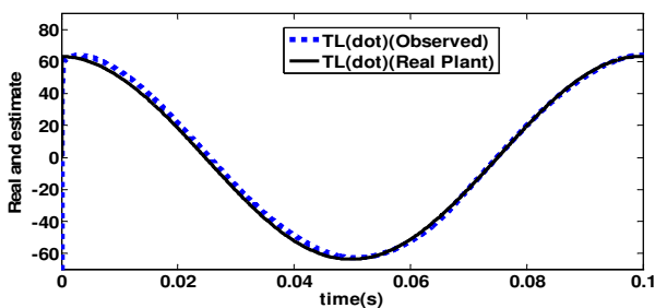
Fig. 8. Observed and estimated load torque derivative
