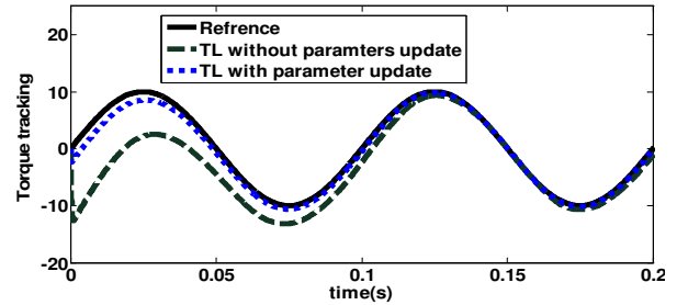
Fig. 9. Torque Tracking without Fuzzy gain Tuning
