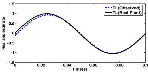
Fig. 7. Observed and estimated load Torque
