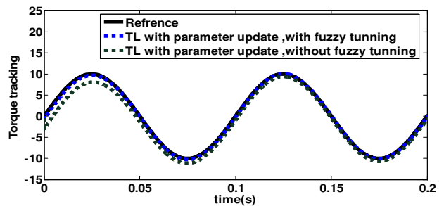
Fig. 10. Torque Tracking with Fuzzy gain Tuning
