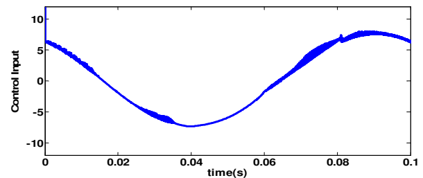
Fig. 11. Control Signal without Fuzzy gain Tuning
