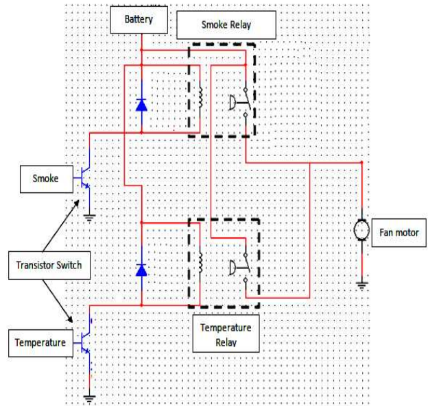
Fig. 5 Smoke and temperature Sensor Circuit
