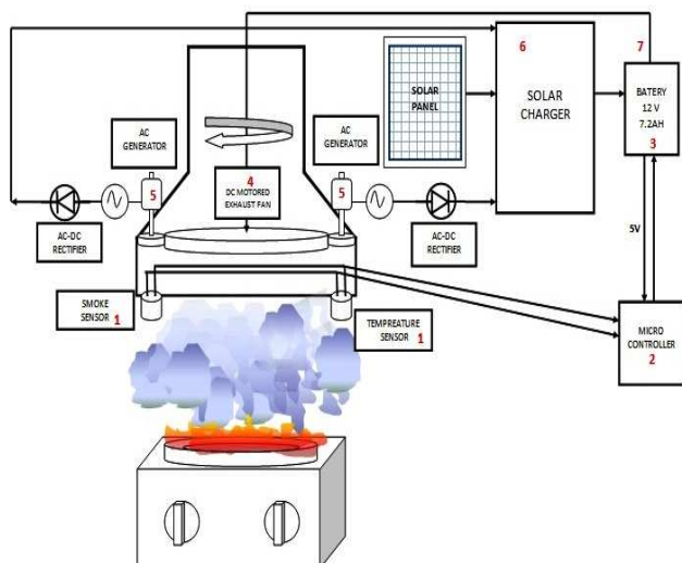
Fig. 1 Configuration of Energy Saving Suction Hood
