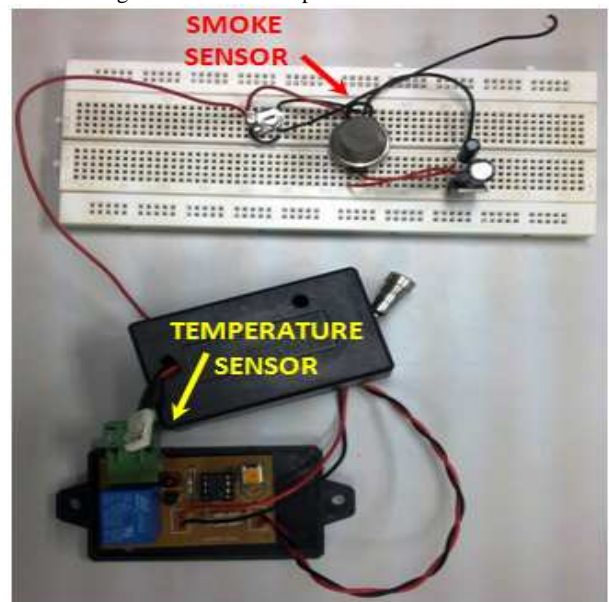
Fig. 6 Smoke and Temperature Sensor
