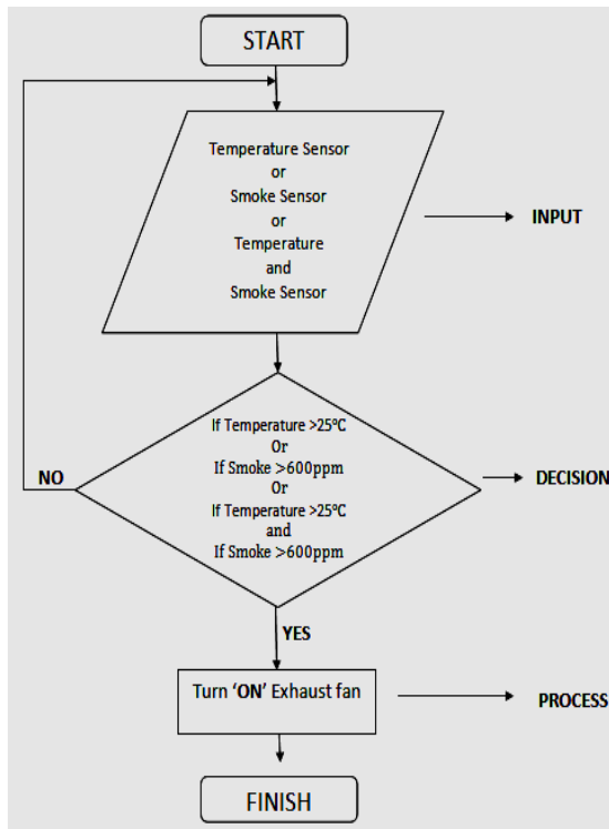
Fig. 4 Flow Chart of Microcontroller Programming
