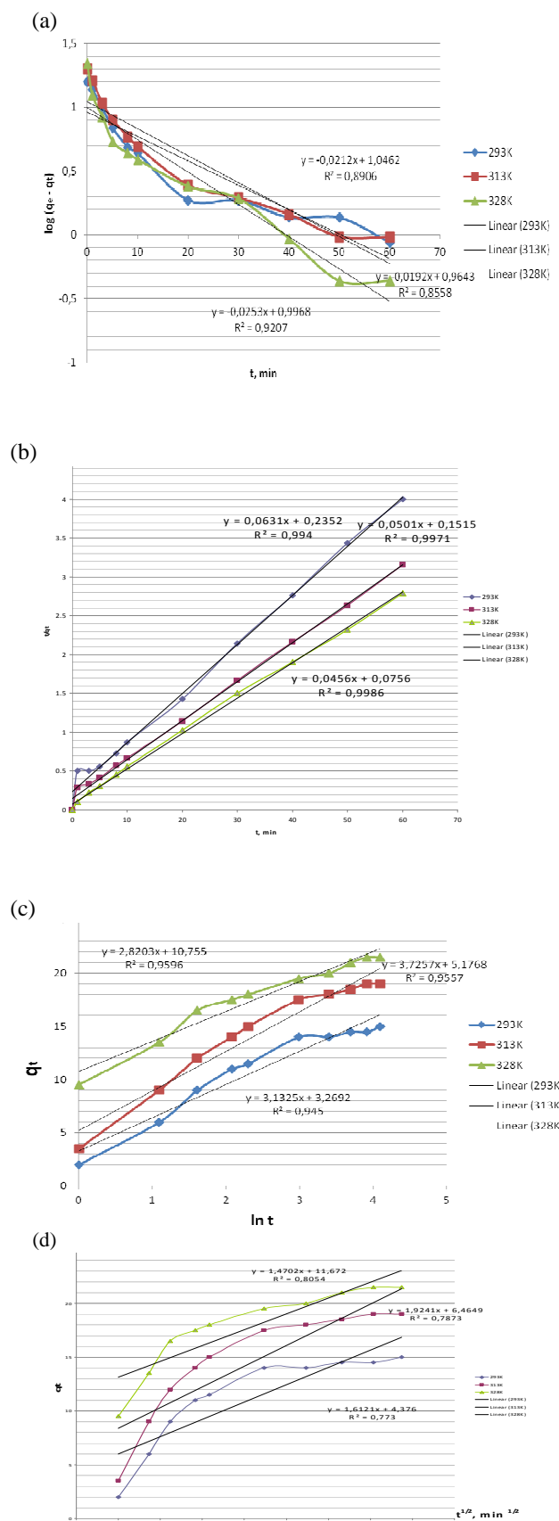
Fig. 3 The plots of the four kinetic models for Cu(II) adsorption onto Zeolite NaA at various temperature
