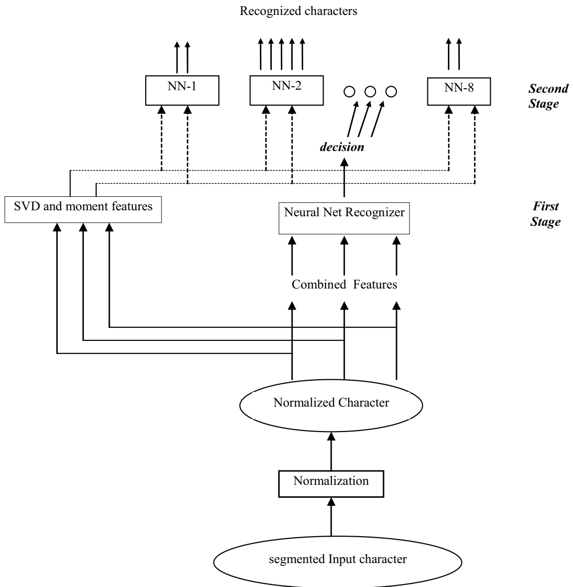
Fig. 3 A new scheme of Arabic character classifier
