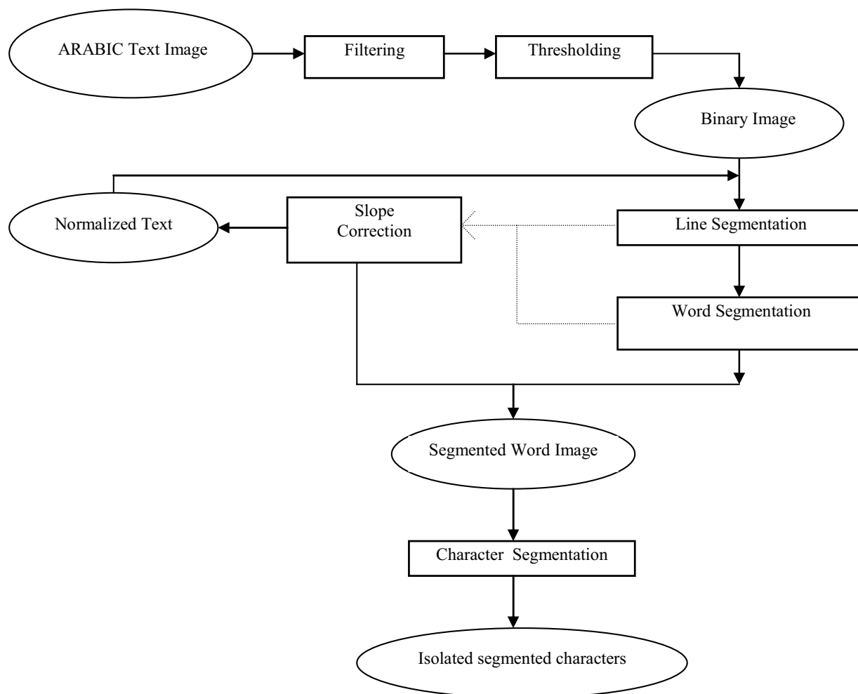
Fig. 2 Overview of the proposed text image preprocessing
