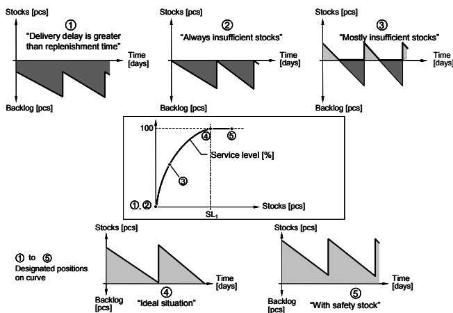
Fig. 3 Development of the service level curve depending on inventory
