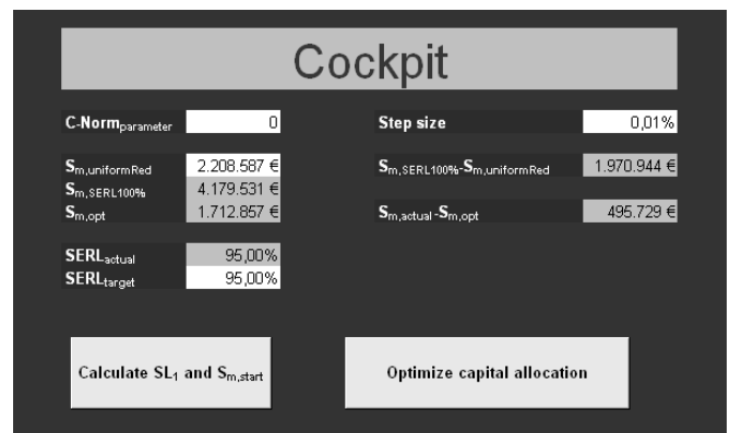
Fig. 6 Software interface
