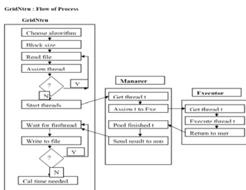
Fig. 2 GridNtru process flow diagram
