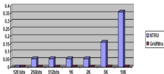
Fig. 5 Decryption performance comparison of NTRU and GridNtru
