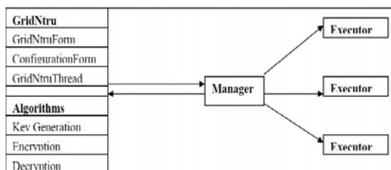
Fig. 1 GridNtru Architecture
