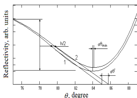
Fig. 11 Comparison of SPR-response for traditional method ( d\theta_{\min} ) and for derivatives method ( d\theta' ). Modeling of presence of biomolecular layer with d_{\text{mol}} = 10\text{nm} on the dielectric layer d_d = 50\text{nm} ( N_d = 1.5 + 0.02i ). 1 – SPR - curve without biomolecular layer, 2 - with biomolecular layer
