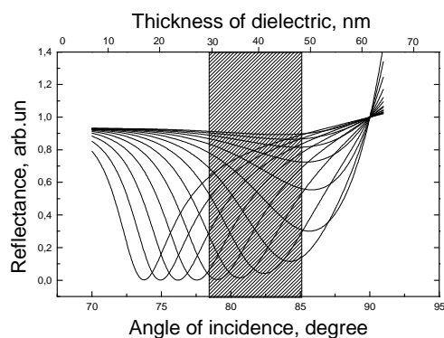
Fig. 10 Calculated SPR-curves for structure Au-dielectric ( N_d=1.5+0i ) for step by step increasing of thickness of dielectric (step 5 nm). Selected angle region – zone of strong increasing of SPR response \Delta\theta_{\min}
