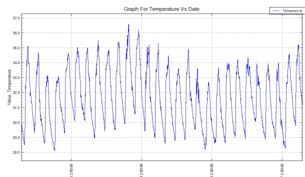
Fig. 8 Temperature Measurement for Feb 2012
