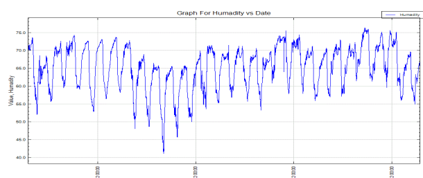
Fig. 7 Humidity Measurement for Feb 2012
