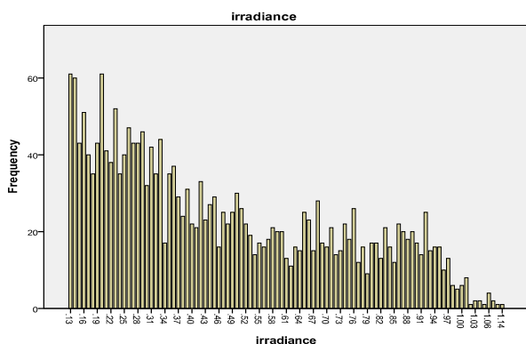
Fig. 10 Irradiance Reading for Day Time
