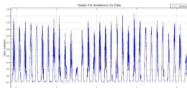
Fig. 4 Peak Irradiance Population for Jan 2012
