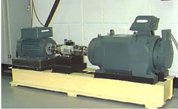
Fig. 6 Experimental setup
