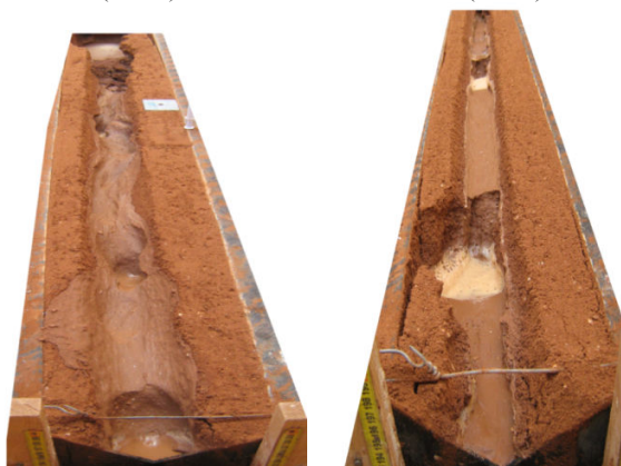
Fig. 4b Types of erosion for circular groove
