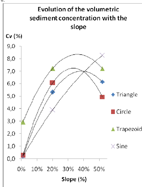
Fig. 5 Evolution of the volumetric concentration
