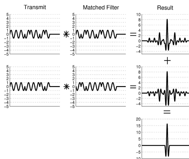
Fig. 3 Principle of side-lobes cancellation using pair of Golay complementary sequences of length 8 bits
