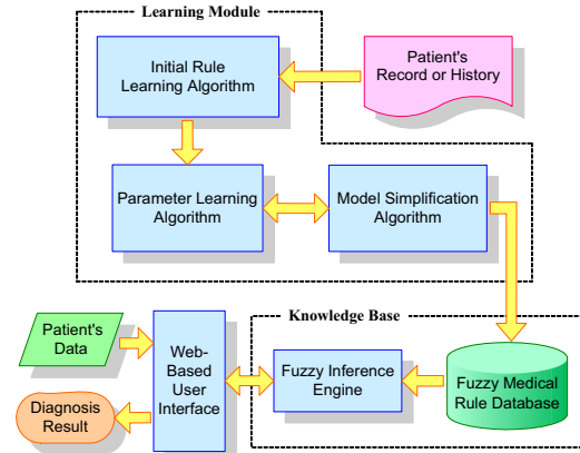
Fig. 2 The system architecture of IMDS
