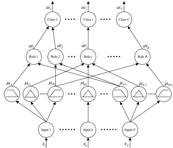
Fig. 1 The architecture of FNN
