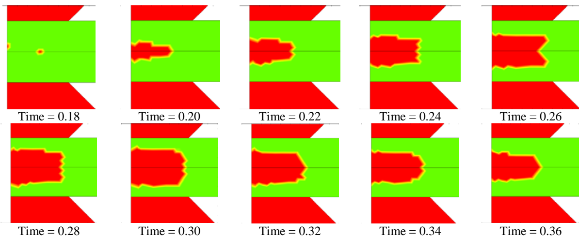
Fig. 5 Welding nugget formation for Case: 1(12.kAmps) with tip area 50.26mm 2
