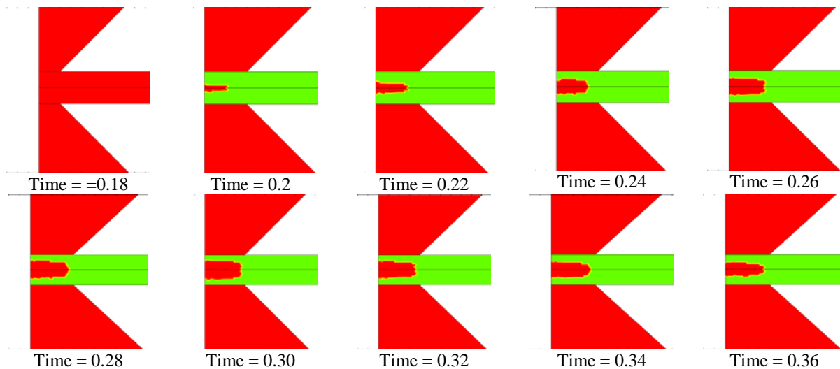
Fig. 12 Welding nugget formation for Case: 3 (19.2kAmps) with tip contact area of 201.06 mm 2
