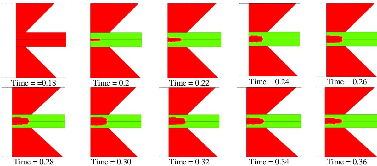
Fig. 9 Welding nugget formation for Case:2 (7.0kAmps) with tip contact area 113.09 mm 2
