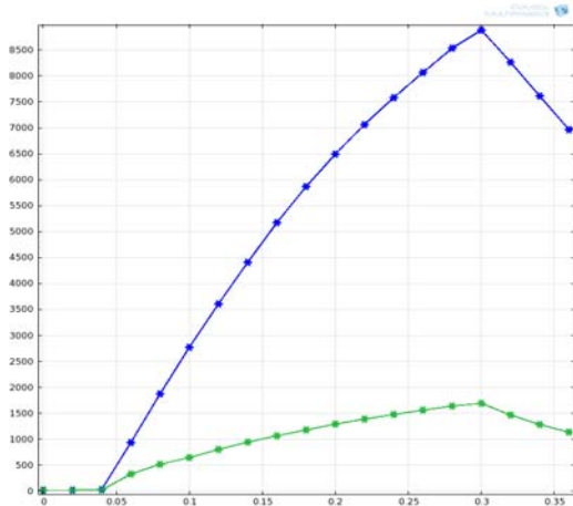
Fig. 6 Temperature changing history at point 1 and point 2 for case: 212.kAmps
