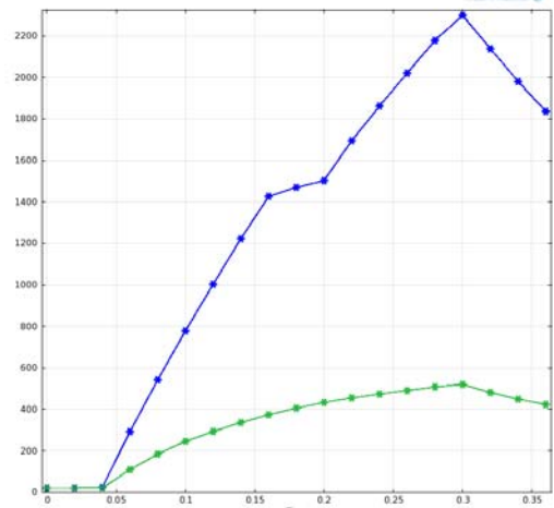
Fig. 4 Temperature changing history at point 1 and point 2 for case :1 12kAmps
