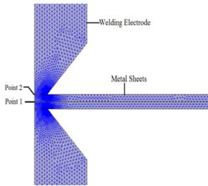
Fig. 2 Geometry meshing
