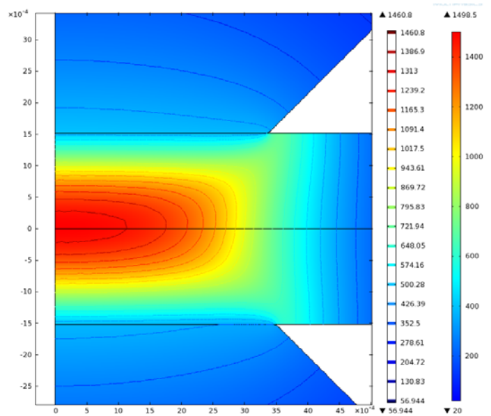
Fig. 3 Thermal profile at faying surface
