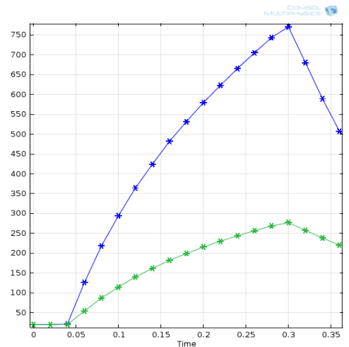
Fig. 10 Temperature changing history at two locations for Case: 3 current 12.2kAmps
