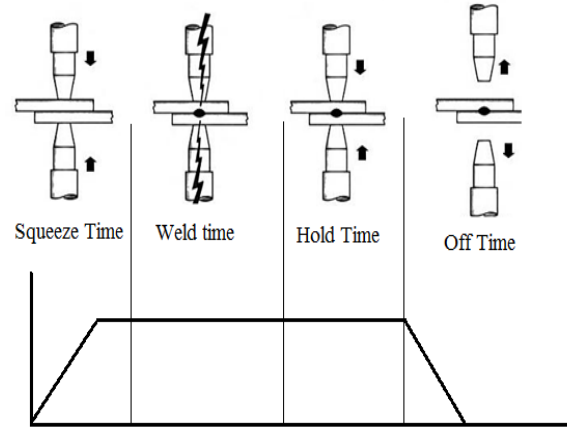
Fig. 1 Complete spot weld cycle
