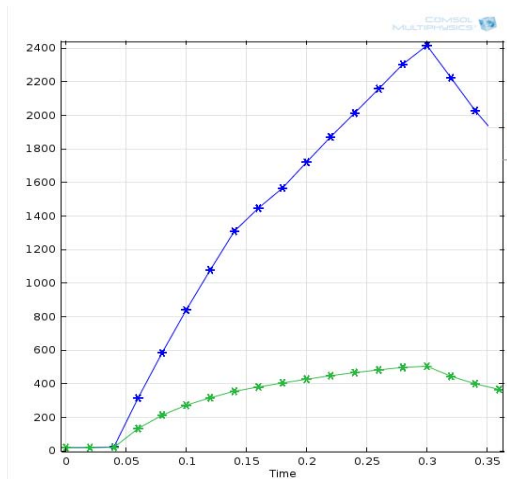
Fig. 8 Temperature changing history at two locations for Case: 2 current 7.0kAmps
