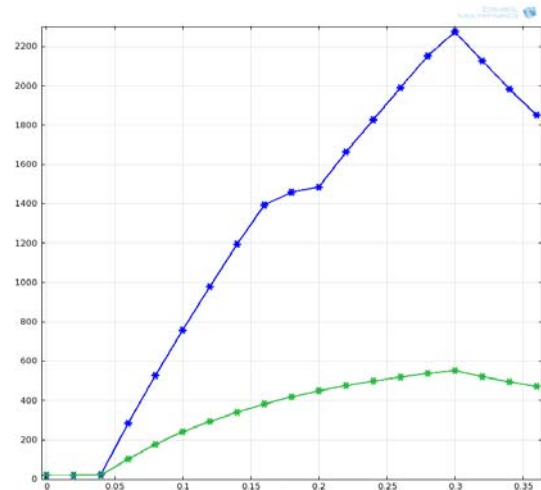
Fig. 11 Temperature changing history at two locations for Case: 3 current 19.2kAmps
