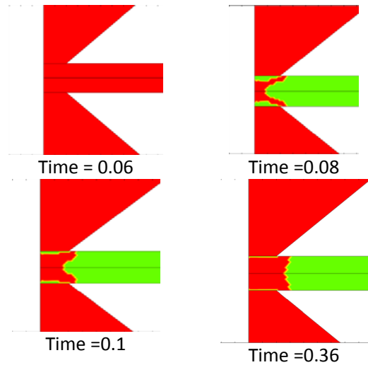
Fig. 7 Welding nugget formation for Case:2 (12.2kAmps) with tip contact area 113.09 mm 2
