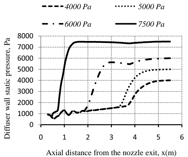
Fig. 8 Static pressure distribution along diffuser wall for back-pressures 4000, 5000, 6000 and 7500 Pa
