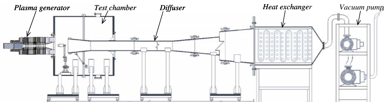
Fig. 1 Schematic of typical plasma wind tunnel
