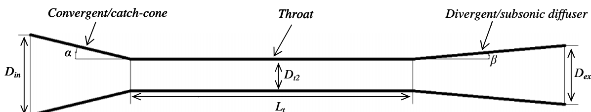
Fig. 2 Schematic of typical supersonic diffuser
