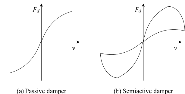
Fig. 3 Curves of velocities-forces for passive and semi-active dampers [5]
