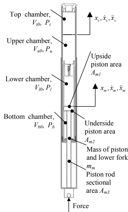
Fig. 7 Mathematical model of the entire damper
