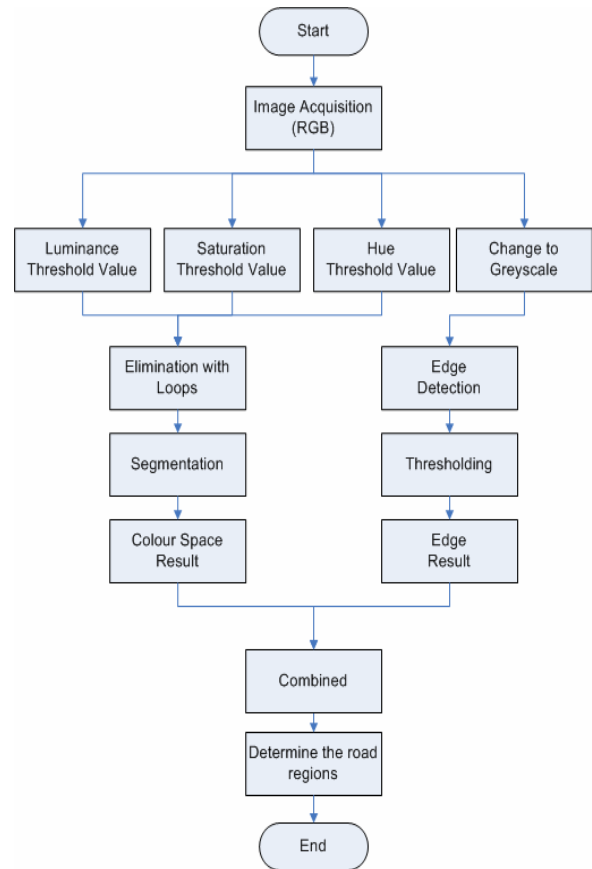
Fig. 1 Flowchart of the hybrid SCSS-EDGE extraction
