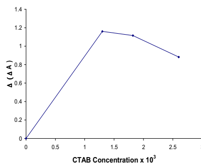
Fig. 4. Effect of CTAB concentration on the sensitivity. Conditions: H_2SO_4 , 0.12M; 5 ng/ml Ru(III); Rhodamin B 5 \times 10^{-5} M; 2.0 \times 10^{-3} M bromate at 27 °C, in fixed time of 0.5–2min from initiation of reaction
