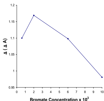
Fig. 3. Effect of bromate concentration on the sensitivity. Conditions: H_2SO_4 , 0.12M; 5 ng/ml Ru(III); Rhodamin B 5 \times 10^{-5} M; 1.2 \times 10^{-3} M CTAB at 27 °C, in fixed time of 0.5–2min from initiation of reaction
