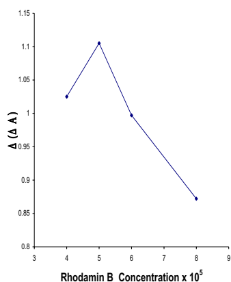
Fig. 2 Effect of Rhodamin B concentration on the sensitivity, conditions: H_2SO_4 , 0.12M; 5 ng/ml Ru(III); 6.0 \times 10^{-3} M bromate and 1.2 \times 10^{-3} CTAB at 27 °C, in fixed time of 0.5–2min from initiation of reaction
