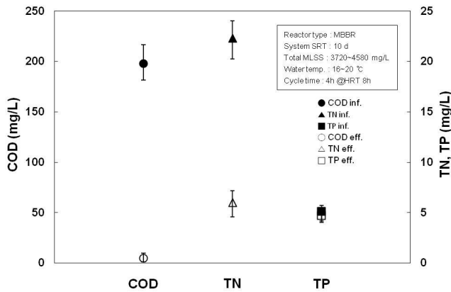
Fig. 1 Removal Efficiency COD, TN and TP
