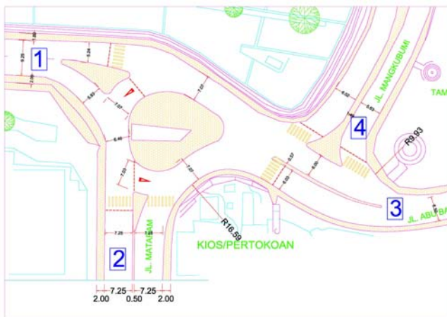
Fig. 4 Kleringan roundabout
