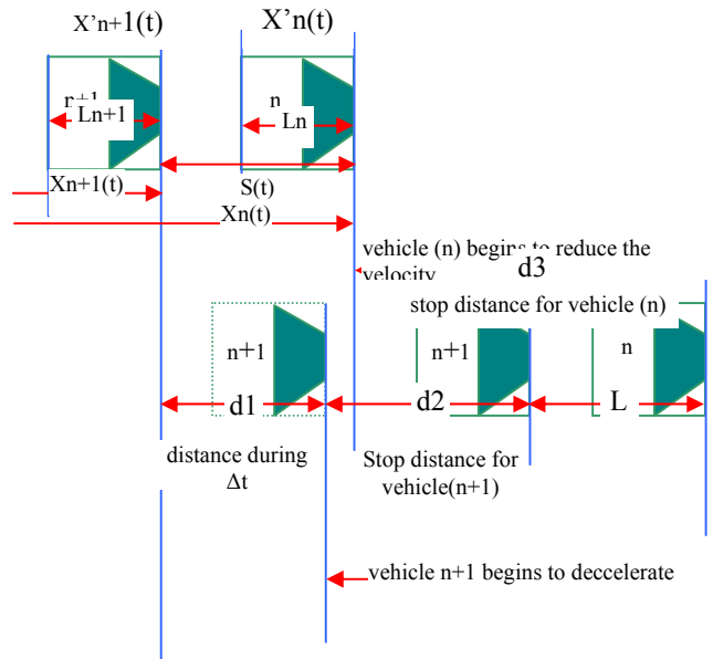
Fig. 3 Vehicle position approaching stop line
