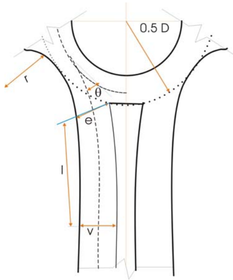
Fig. 2 Roundabout Geometry
