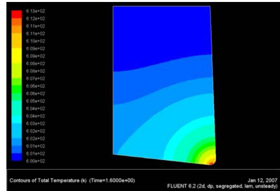
Fig. 4 Temperature distribution in heat transfer analysis by FLUENT for HSS tool with rake angle of 2°
