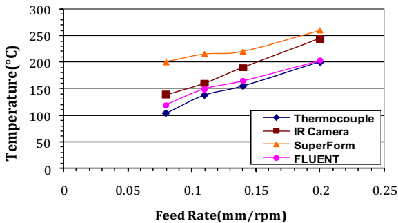
Fig. 18 Diagram of temperature vs. feed rate
